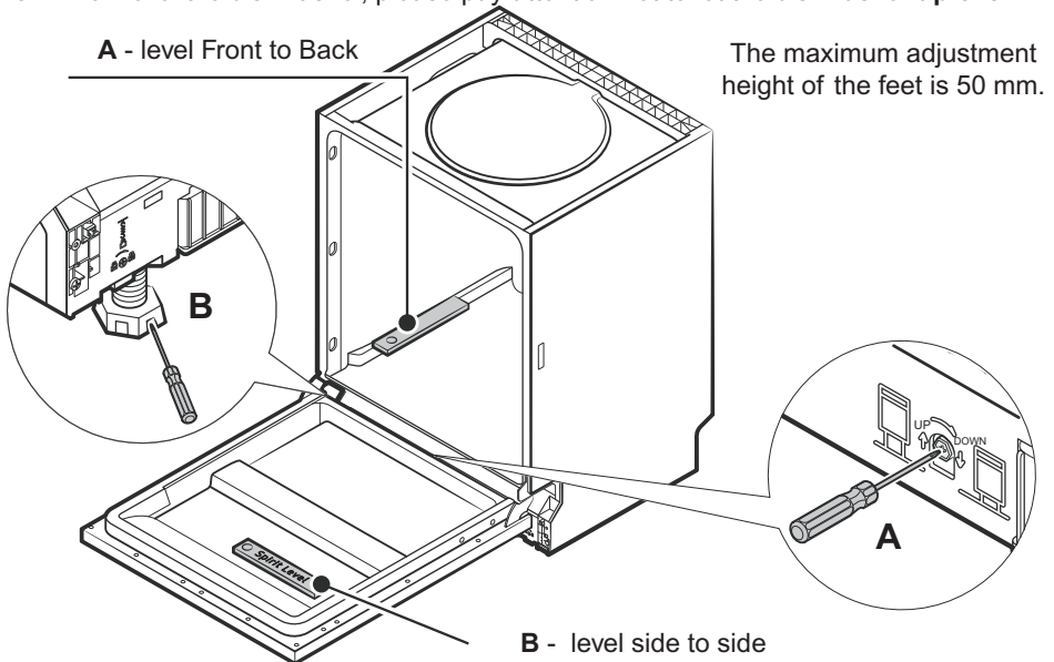
Figure 6 - Dishwasher leveling
